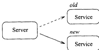
Figure 3: Class Server redirects to a new version of Service class
