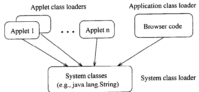
Figure 2: Class loaders in a web browser
